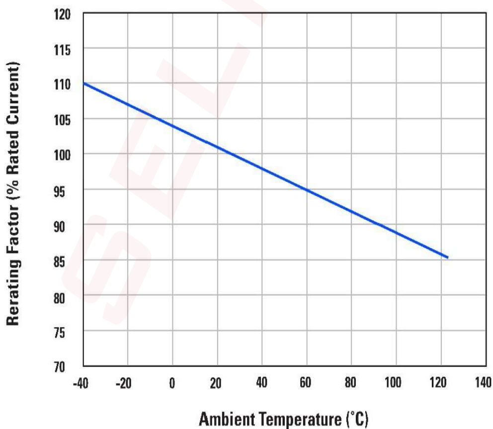
Temperature Rerating Curve
